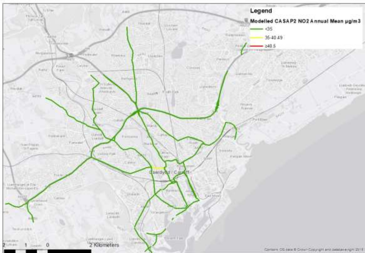
Figure 16 Sampled NO 2 results along the PCM links > 35 µg/m 3 for CASAP 2 in 2021
