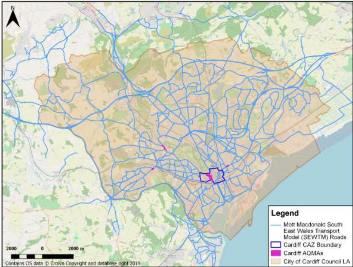
Figure 3: CAZ study domain and relationship to Mott Macdonald’s sub-regional transport model links
